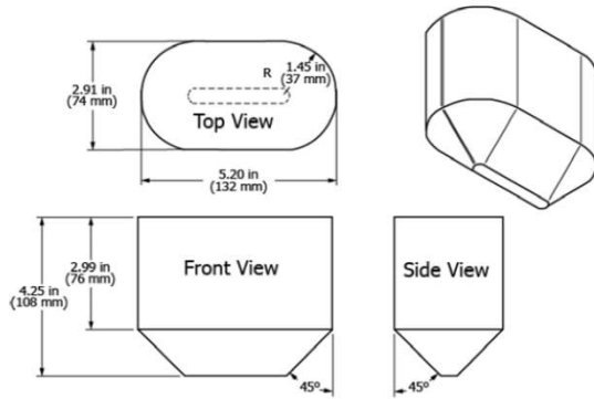
FIG. 7 Modified Bath Seat Torso Probe
